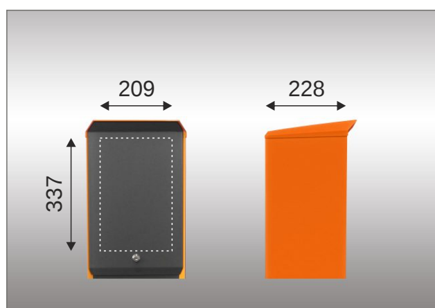
Installation dimension Terminal MS and ML
