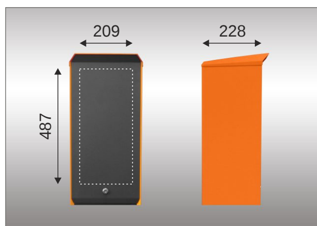
Installation dimension Terminal MH
