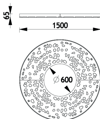
Pebbles Ø1,50 m Ref: 42 25R04 GR 108 kg
