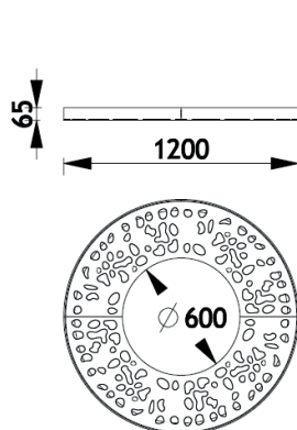
Pebbles Ø1,20 m Ref: 42 22R04 GR 60 kg
