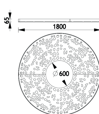
Pebbles Ø1,80 m Ref: 42 28R04 GR 149 kg
