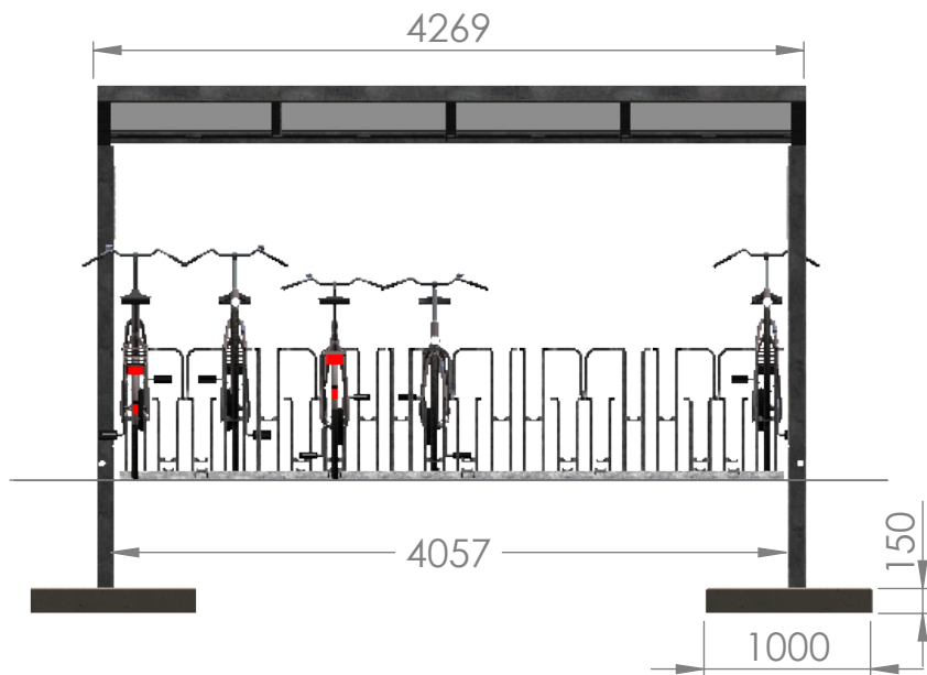
T-Hide double-sided 1 section - h.2.h. 400 mm
