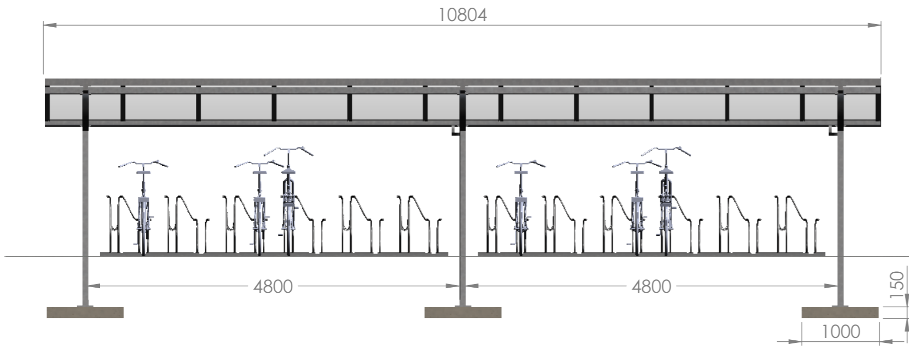
Top single-sided 2 sections - h.2.h. 375 mm
