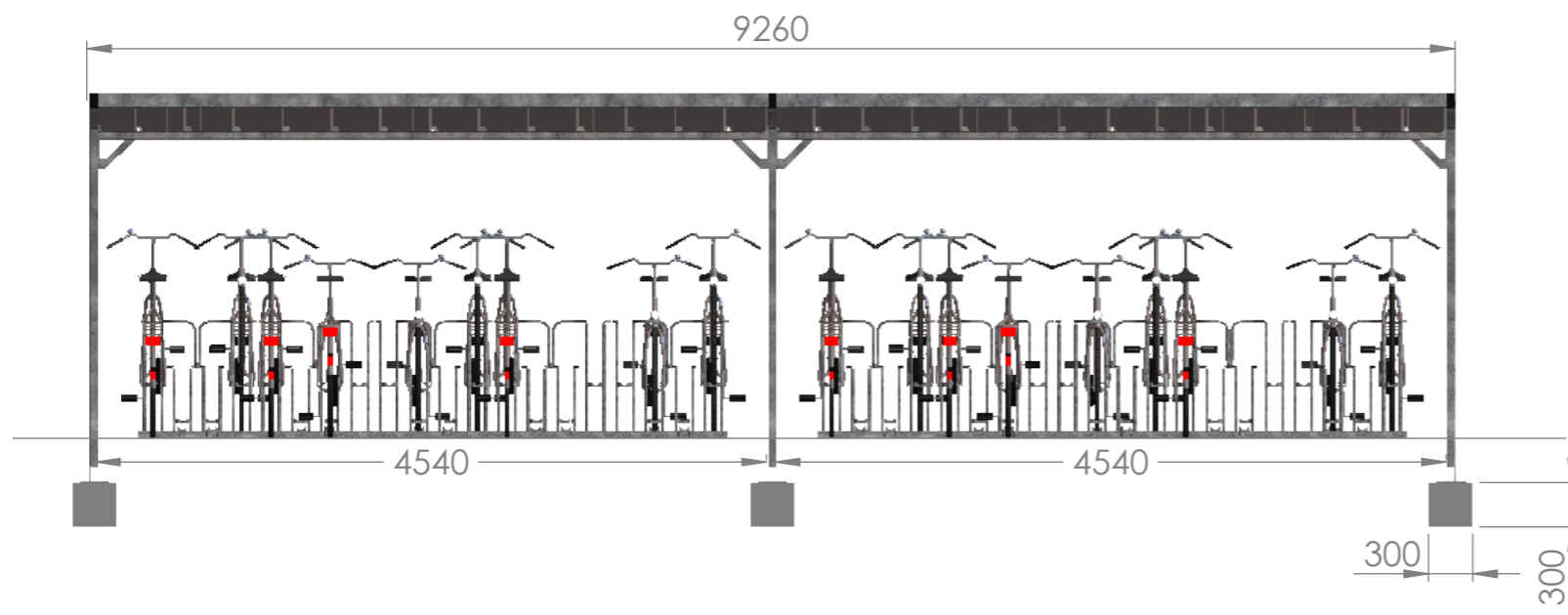
Wave double-sided 2 sections - h.2.h. 400 mm
